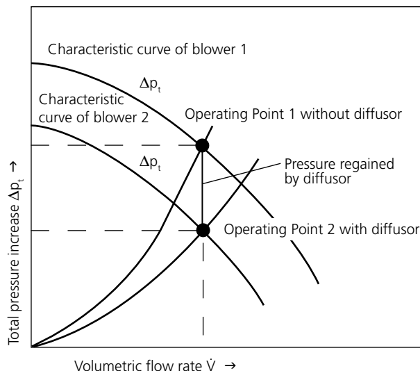
Figure 2: Pressure recovery
