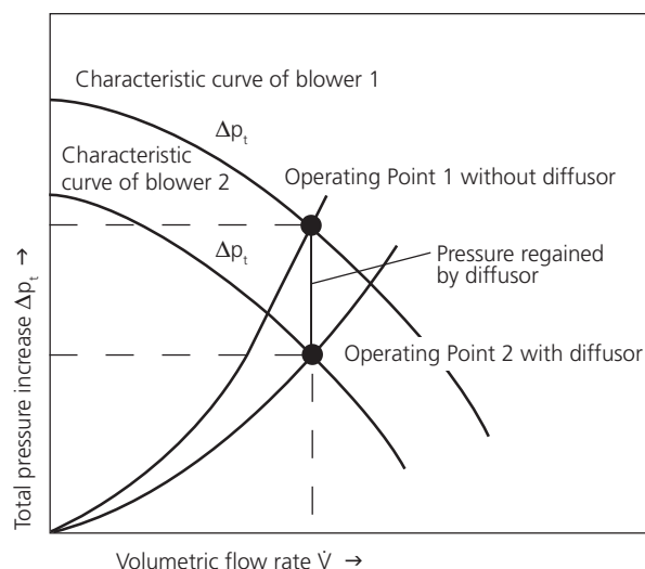
Figure 2: Pressure recovery
